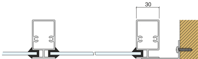
Toppvy fast B-parti
